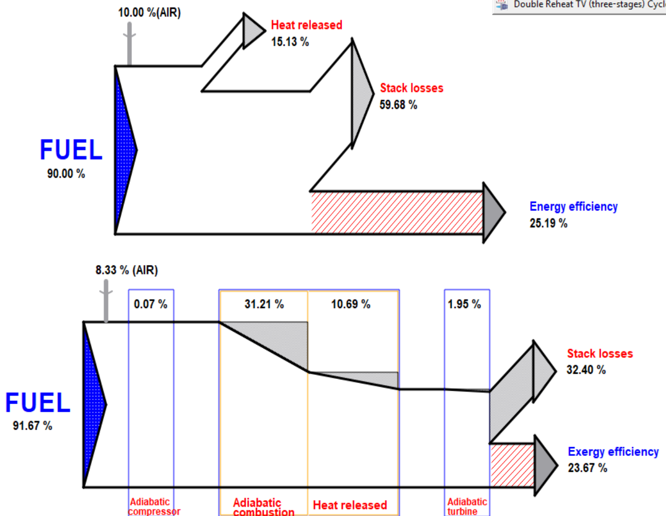
Results visualization using a Grassmann combustion diagram
